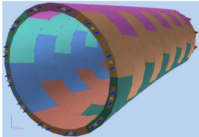
3D design of the 80m radius segments.
